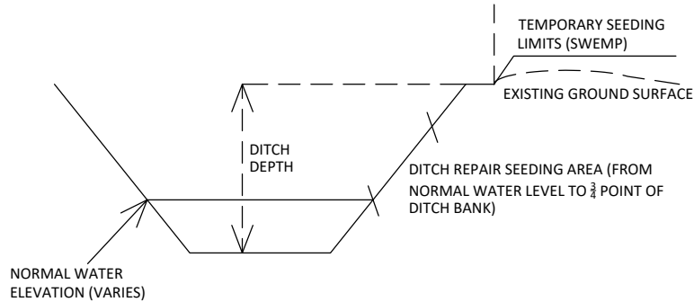
AREA OF SEEDING FOR DEPTH OF DITCH AND PORTION OF VEGETATION REMOVED (SF PER STATION PER SIDE) FOR SIDESLOPE 1.5:1
