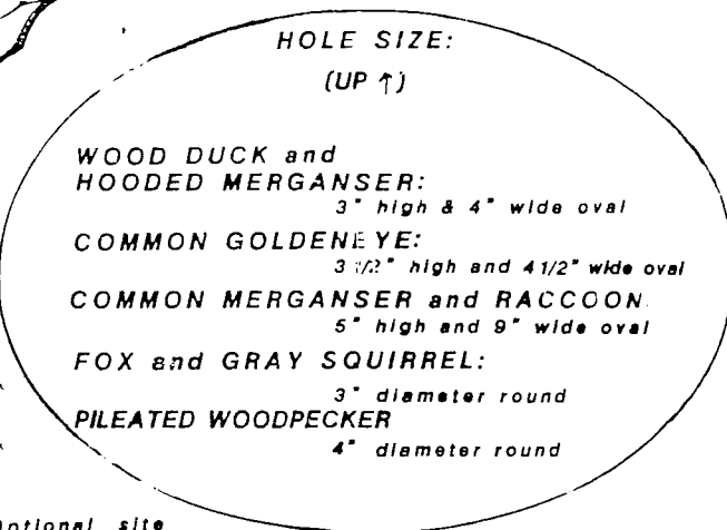
FIGURE 14. WOOD DUCK HOODED MERGANSER COMMON GOLDENEYE COMMON MERGANSER RACCOON FOX and GRAY SQUIRREL PILEATED WOODPECKER (?) NEST BOX
