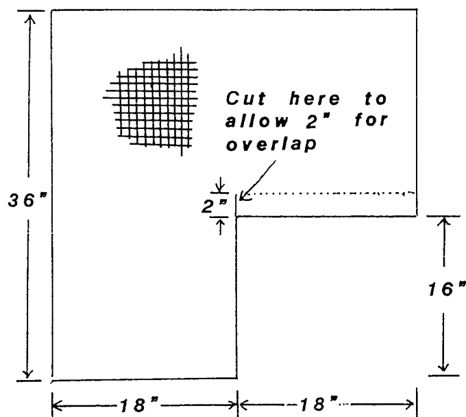
Basket Pattern 1/2" mesh hardware cloth
